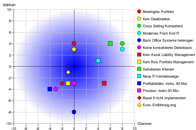
Relato: SWOT-Analyse
